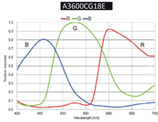
Quantum Efficiency Curve for Mono and Color
