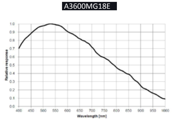
Quantum Efficiency Curve for Mono Sensor
