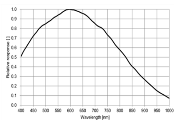
Mono Spectral Response Sony IMX 253
