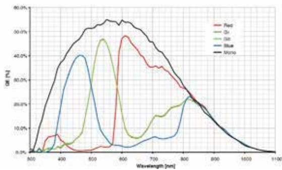
Quantum Efficiency Curve for Mono and Color
